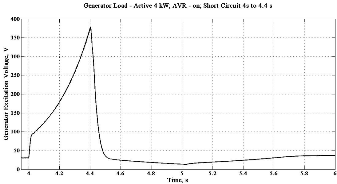
Fig. 6. Excitation voltage of the synchronous generator
