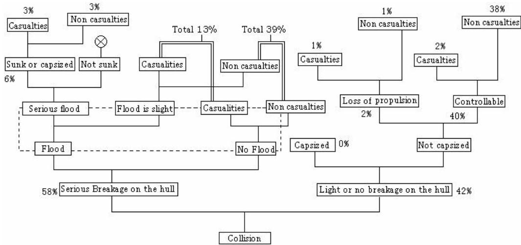
Fig.2. Event Tree of existence of casualties
