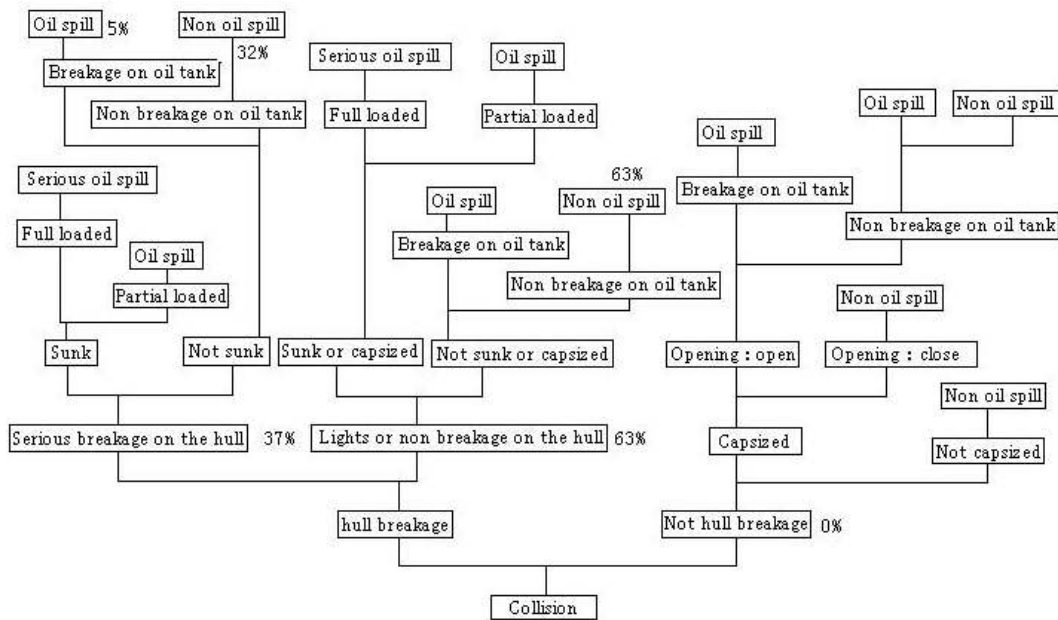
Fig.1 Event tree of the tanker
