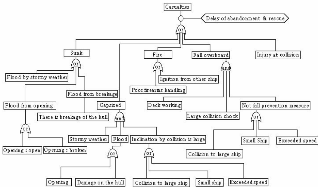
Fig.3. Fault Tree of existence of casualties
